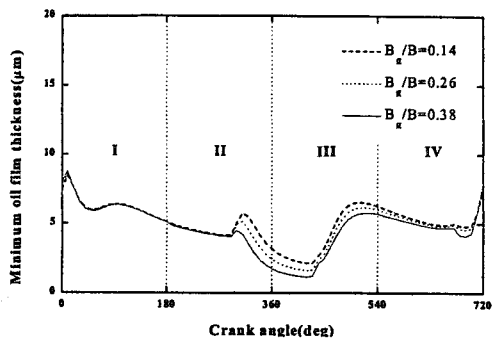
Fig. 10 Calculated results of MOFT for various groove widths in No. 1 main bearing (3500rpm, C=20 \mu\text{m} , 180° half groove)
