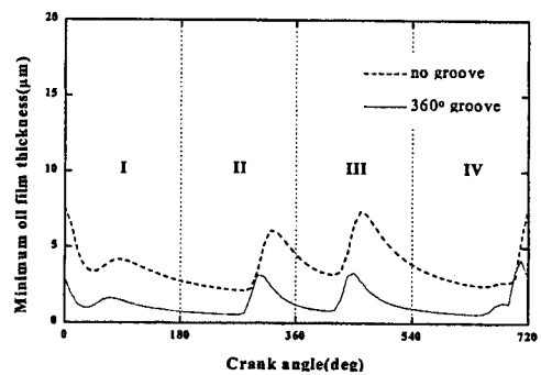
(a) 3500 rpm
