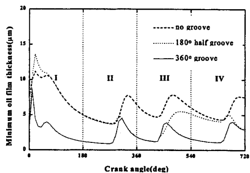
Fig. 11 Calculated results of MOFT curves in No. 1 main bearing (5500rpm, B_g/B=0.26 , C=20 \mu\text{m} )
