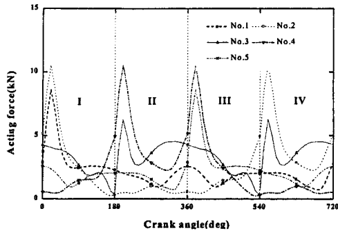
Fig. A1 Resultant acting forces on the main bearings (3500 rpm)
